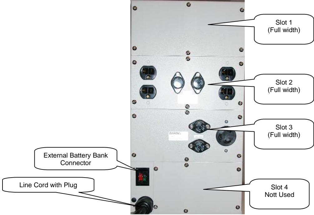
SG 5 & 6kVA PDU View of Rear Panel Mounted PDU (typical)
